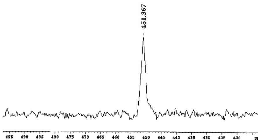
(ii) \text{PW}_{11}\text{O}_{39}\text{Co}
